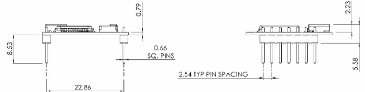
Figure 3: Side Views
