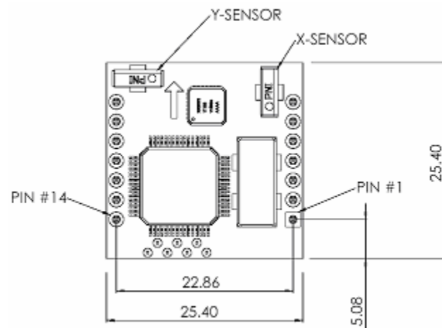
Figure 4: Top View
